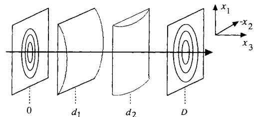
FIG. 1. Wave field in the x_3=0 plane propagates through two cylindrical lenses, oriented along the x_1, x_2 directions, and is detected in a plane at x_3=D . Intensity data are collected for many combinations of focal lengths f_1, f_2 and distances d_1, d_2 .
